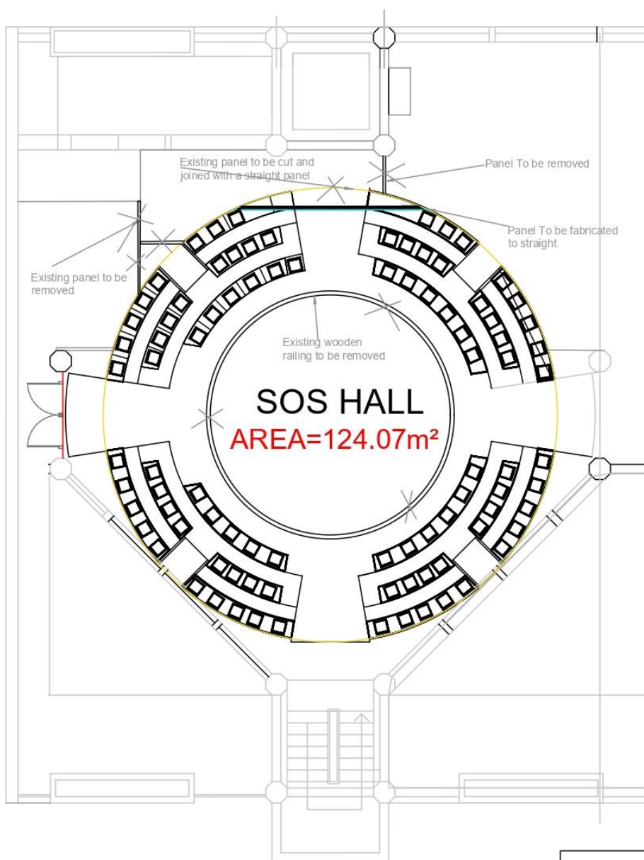
Existing Layout
