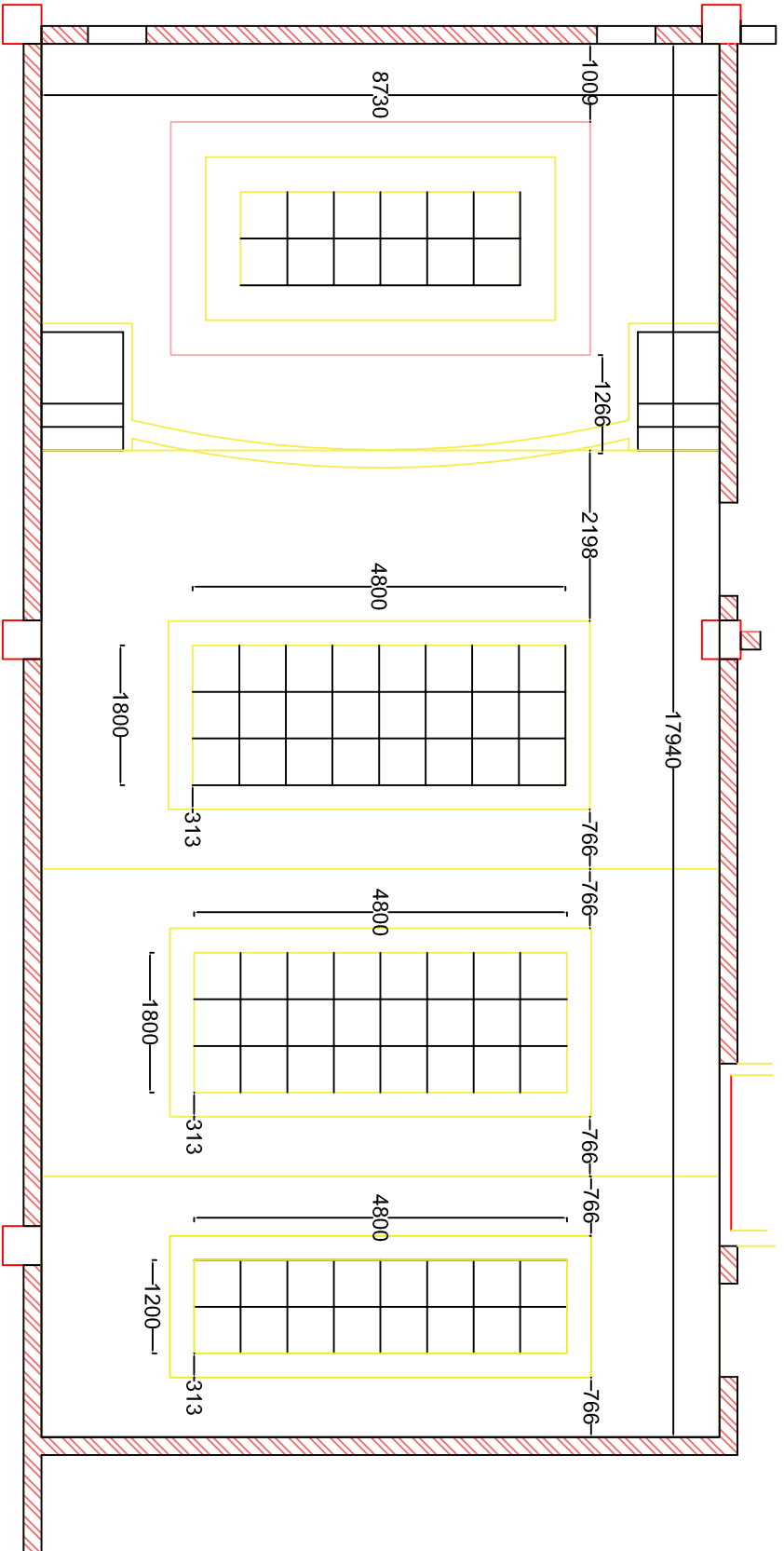
AUDITORIUM FALSE CEILING PLAN
